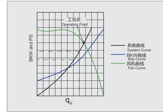
Fig.4 Operating Point
