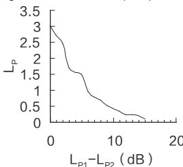
Fig 1. Two noise sources superimposed curve
