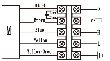
SINGLE-PHASE DOUBLE SPEED WIRING DIAGRAM
