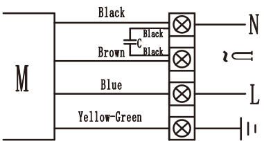
SINGLE-PHASE WIRING DIAGRAM
