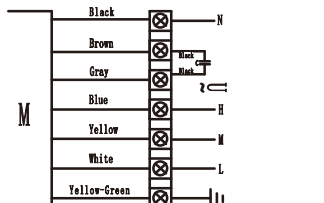
SINGLE-PHASE THREE SPEED WIRING DIAGRAM
