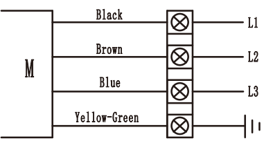
THREE-PHASE WIRING DIAGRAM
