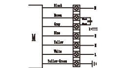
SINGLE-PHASE THREE SPEED WIRING DIAGRAM
