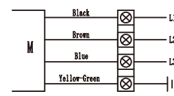
THREE-PHASE WIRING DIAGRAM
